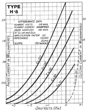
Characteristic Curve of Average H.8 Valve.
